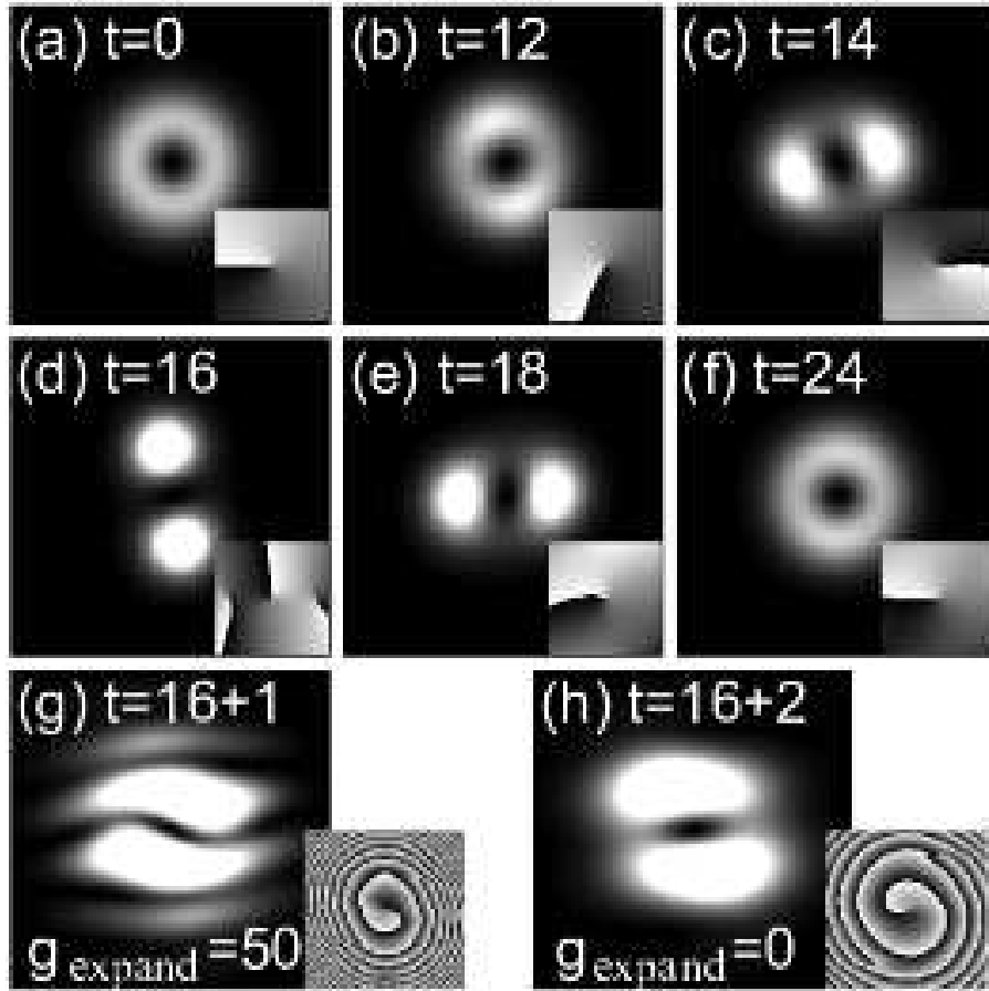
Fig. 9. Nonlinear dynamical split-merge cycle of bright ring soliton. (a)-(f) Shown is the time evolution of the density profile in two dimensions. The insets present grey-scale plots of the phase modulo 2\pi . Panels (g) and (h) show what occurs when the trap is switched off and the condensate is allowed to expand with (g) large positive scattering length and (h) zero scattering length. This is a common experimental technique to magnify condensate features too small to otherwise resolve.
