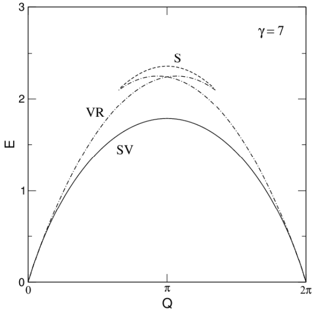
Fig. 4. The energy E versus impulse Q dispersion relation of the known solitary waves in the cylindrical BEC at \gamma = 7 from Ref. [47]. Shown are the branches of the svortex (SV), vortex rings (VR), and the band soliton (S). The slope dE/dQ of the dispersion relation gives the velocity of the solitary wave. The density structure of vortex rings and the time-dynamics of their head-on collision is shown in Fig. 5.
