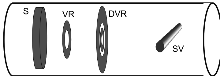
Fig. 3. Schematic of solitary wave configurations in a cylindrical BEC. The band soliton (S) has a nodal plane perpendicular to the trap axis and shows axial and inversion symmetry. The vortex ring (VR) is axisymmetric and has a vortex line (line singularity in the phase) in the configuration of a closed ring around the trap axis. The double vortex ring (DVR) has the same symmetries as the VR but features two concentric loops of vortex lines. The solitonic vortex (SV) has no symmetry. A vortex line is configured perpendicular to the trap axis and does not close in itself but terminates at the condensate boundaries.
