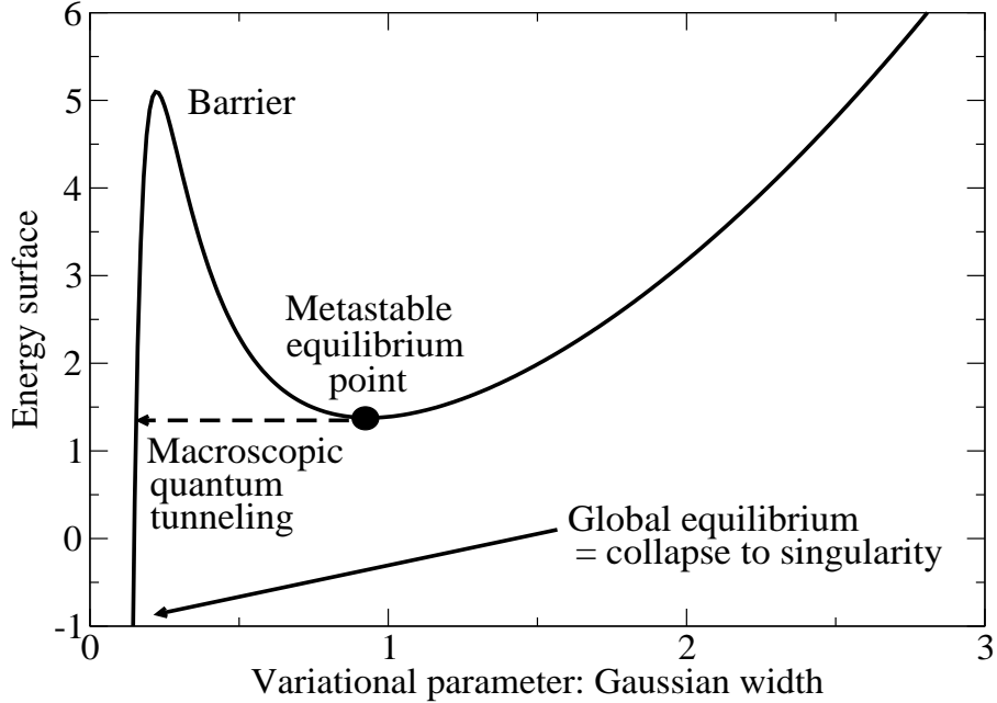
Fig. 7. Metastability and macroscopic quantum tunneling: Shown is a representative energy surface for a variational Gaussian ansatz in an isotropic 3D harmonic trap for attractive interactions g_{\text{eff}} < 0 , as a function of the single variational parameter, the width of the Gaussian. One observes that non-singular solutions (non-zero width) are always metastable. The height of the collapse barrier decreases as N \rightarrow N_c^- ; N_c is the critical number of atoms for which the barrier disappears and collapse is driven classically. Macroscopic quantum tunneling towards collapse can also occur through the barrier, as sketched on the plot [78].
