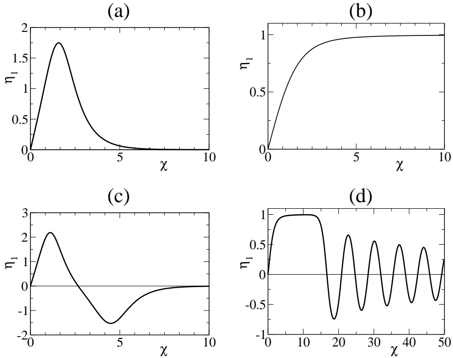
Fig. 2. A quantum vortex of winding number q = 1 in free space: (a) attractive case; (b) repulsive case. It is evident in (a) that a bright vortex is also a bright ring soliton. A radially excited state: (c) the first excited state in the attractive case; (d) in the repulsive case, a radially excited state requires an infinite number of nodes and asymptotically resembles the Coulomb function [32]. The radial dependence of the order parameter of an infinitely extended condensate is depicted. Note that all axes are dimensionless: \eta_1 is a rescaled radial density while \chi is a rescaled radial coordinate.
