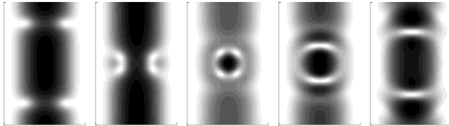
Fig. 5. Inelastic collision of vortex rings produces a transient shell structure of near spherical symmetry, from Ref. [44]. Plotted is the density |\Psi|^2 on the y = 0 plane at different time frames showing the head-on collision of a pair of vortex rings at \gamma = 7 with v \equiv dE/dQ = 0.34v_s , where v_s = 1.61 is the speed of sound in the units of Eq. (3).
