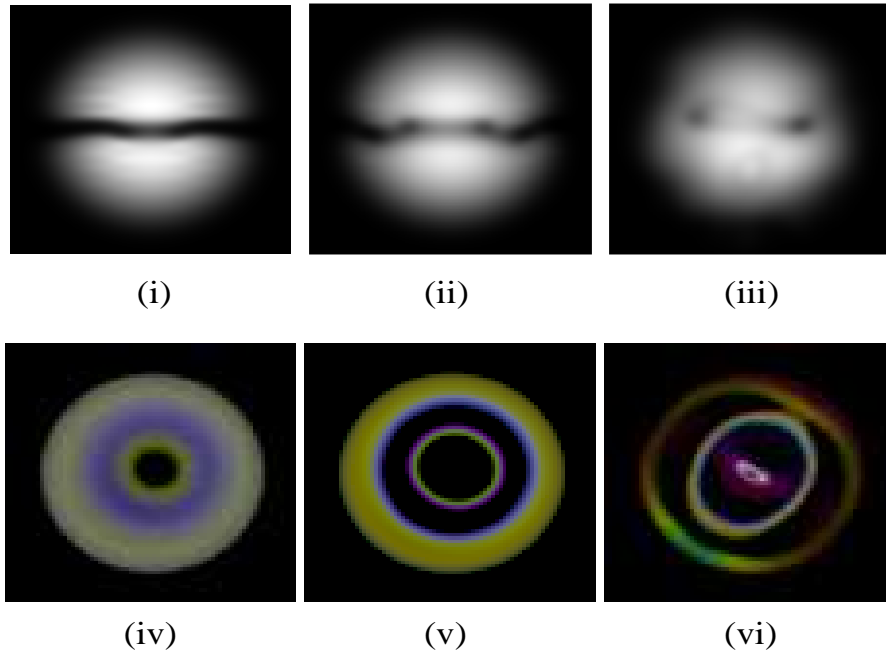
(a) Snake instability in a spherical trap
