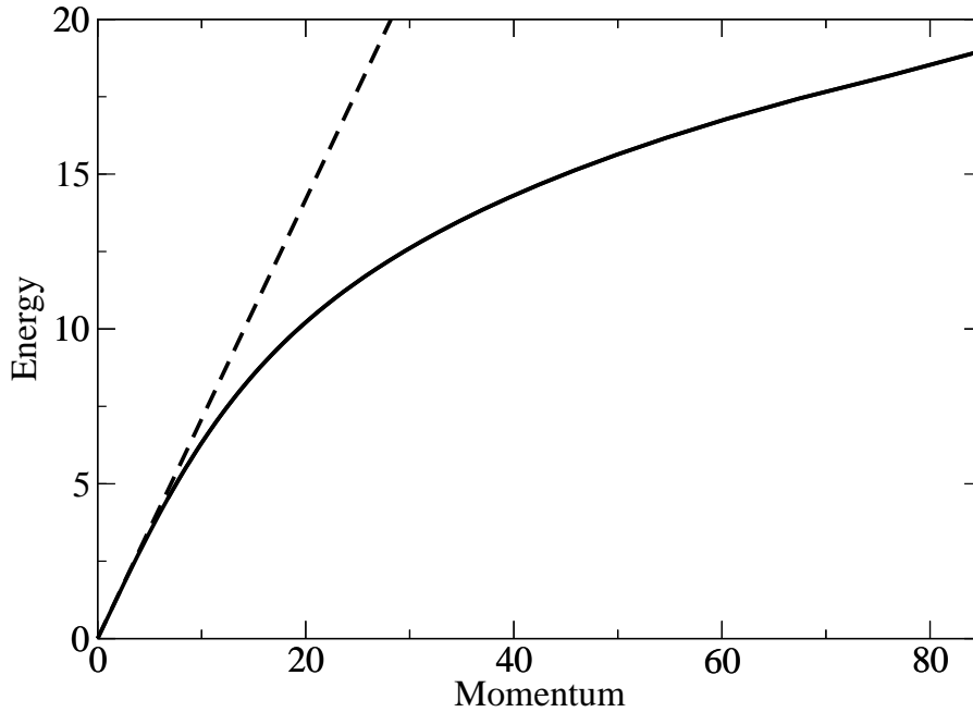
Fig. 6. Dispersion relation [11, 50] for 2D ( xz ) solitary waves (solid line). The dashed line shows the dispersion relation of sound for comparison.
