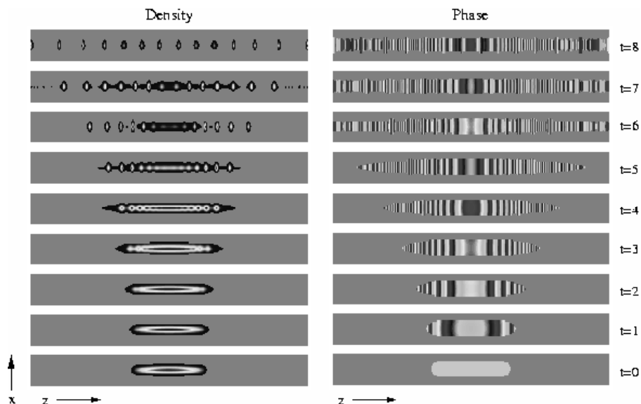
Fig. 8. Pulsed atom soliton laser: An initial state created by changing the scattering length of a condensate from large and positive to small and negative and then projecting the condensate on to an expulsive harmonic potential results in spontaneous modulational instability and a series of phase-coherent pulses, or “mini-BECs.” Shown are the evolution of the density and phase along a two dimensional cut at y = 0 . A set of well-defined solitonic pulses is evident in the latest (top) panel. The strong variations in the phase at late times is due to the high momentum of the solitons caused by the expulsive harmonic potential. Note that the phase is shown on the color circle, i.e. , modulo 2\pi , while the density is in arbitrary relative units rescaled for each plot. For N = 10^4 atoms, a = -3a_0 , and a trap geometry of \omega_\rho = 2\pi \times 2.44 kHz, \omega_z = 2\pi i \times 2.26 Hz, the time units are scaled to 22 ms and the spatial units to 10 \mu\text{m} . Note that the aspect ratio of the plots showing a region of 0.822 by 153 length units was changed for visualization.
