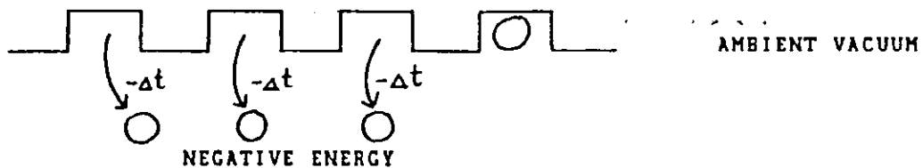
FIGURE 6. The Partially-Emptied Dirac Sea
