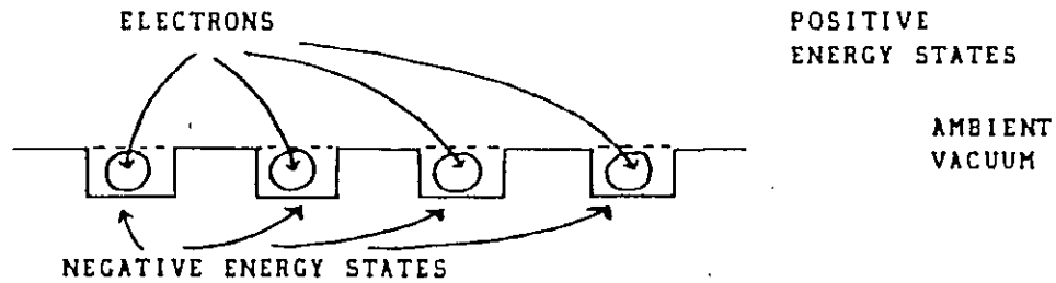
FIGURE 5. The Normally-Filled Dirac Sea
