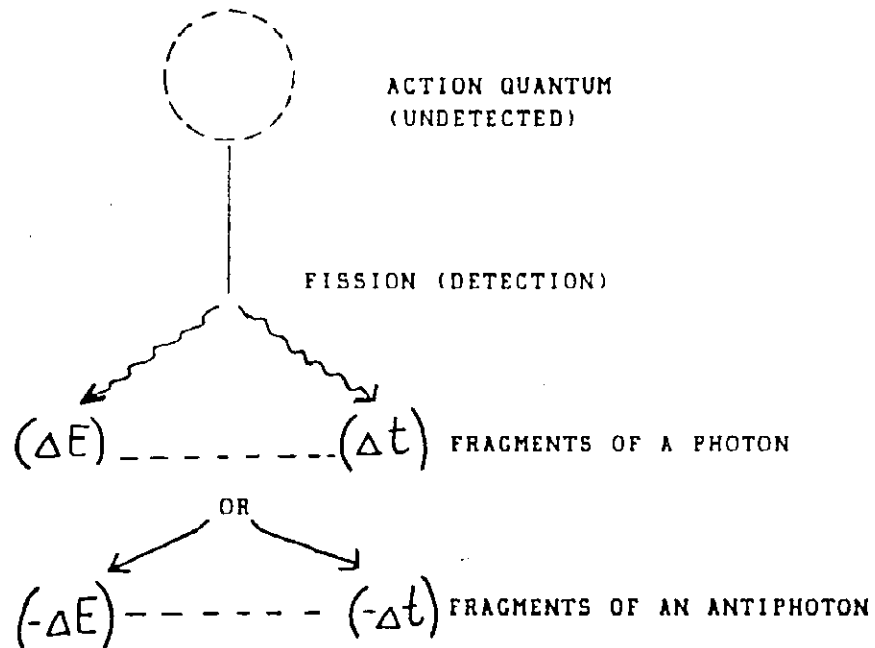
FIGURE 3. Two Possibilities of Action Quantum Fissioning
