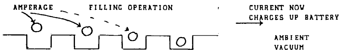
FIGURE 7. Filling The Dirac Sea Holes
